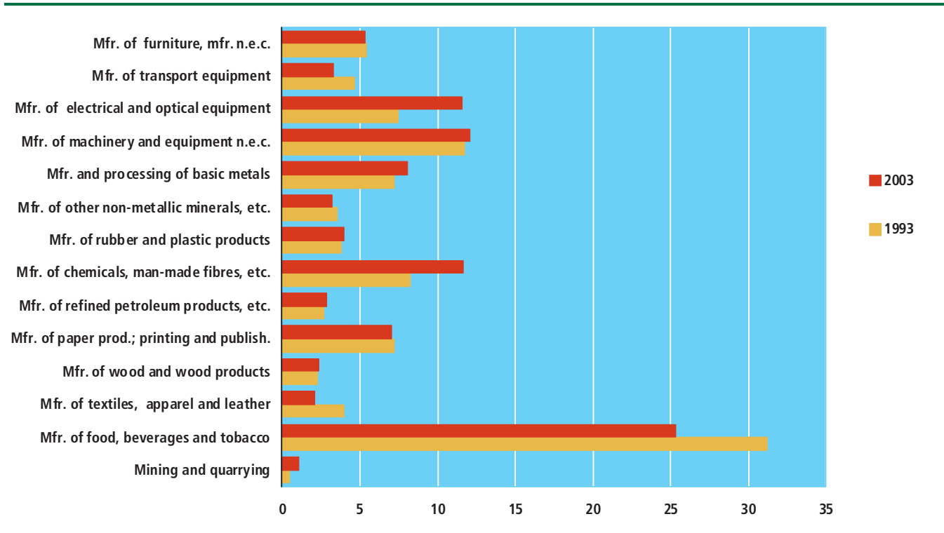
Figure 3 Manufacturers' total turnover by groups of industries, per cent
